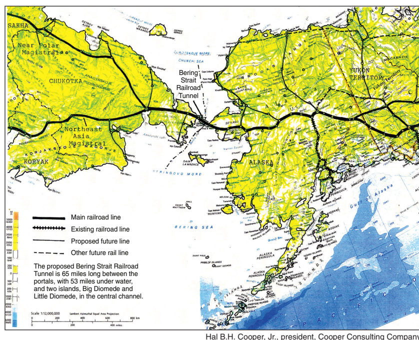
FIGURE 7 Bering Strait Tunnel
