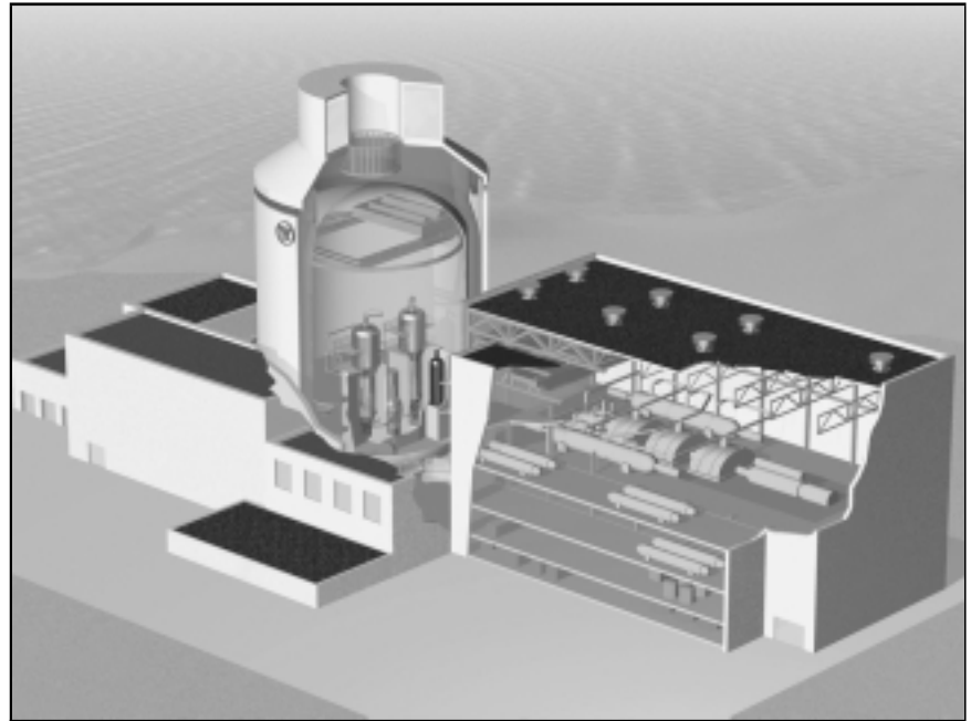
FIGURE 3 Westinghouse AP1000
