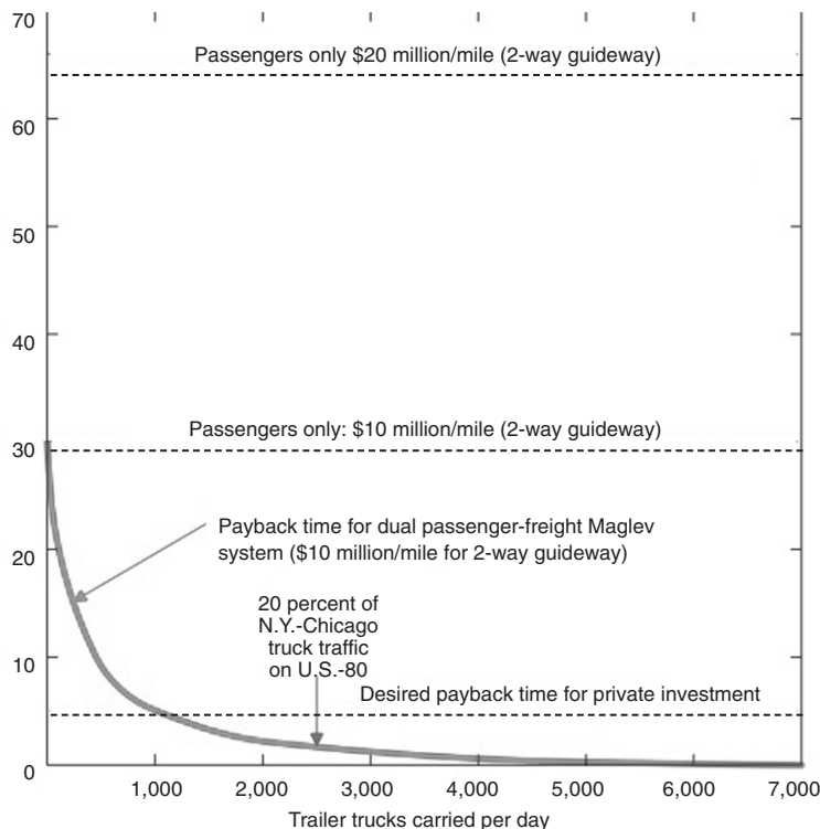
FIGURE 3 Economic Advantages of Maglev Carrying Both Passengers and Trucks
