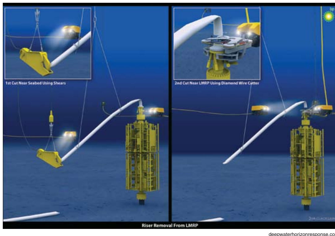
FIGURE 1 Lower Marine Riser Package
