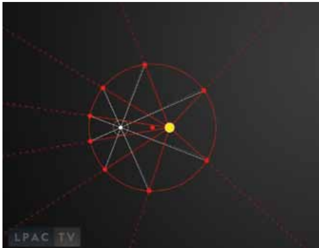
FIGURE 2 A Model of Kepler's 'Vicarious Hypothesis'
