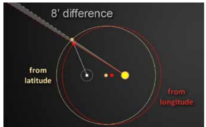
FIGURE 4 The 'Crack': The 'Eight Minutes of Arc'
