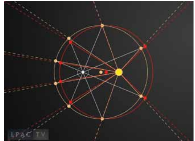
FIGURE 3 Kepler's 'Adjusted' Hypothesis
