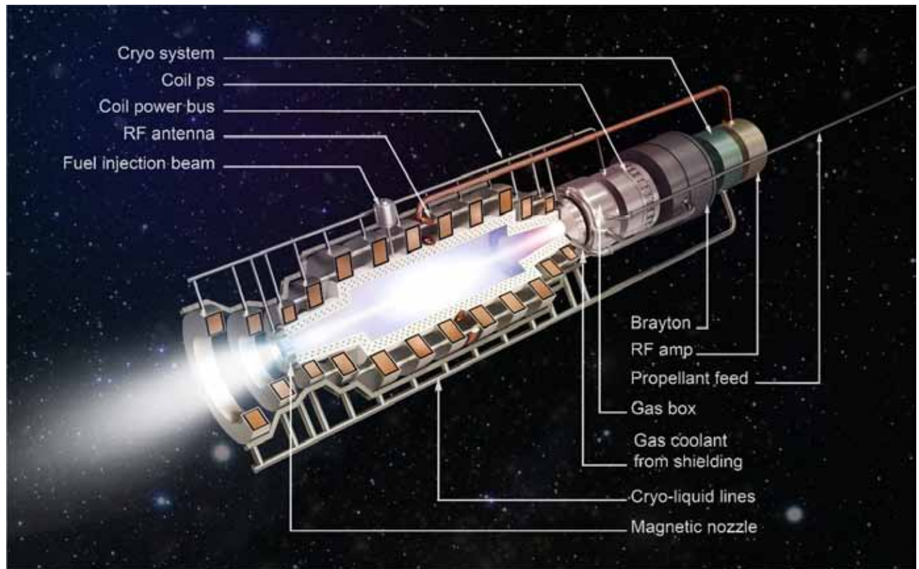
Artist's rendering of a Direct Fusion Drive engine with interior cutout to show detail of the magnetic coils.
