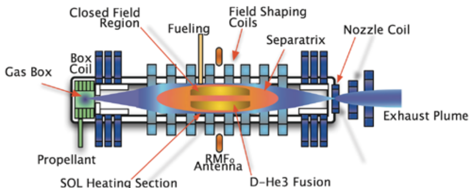
Schematic of Direct Fusion Drive core. Deuterium gas, introduced into the gas box, is ionized there. This newly formed plasma flows to the right in the scrape-off layer (SOL), where the electrons are heated as they pass over the field-reversed configuration region.
